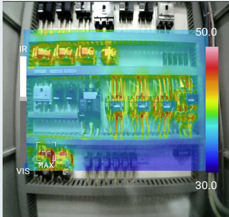
Real-time mixing display of visible & thermal imaging *Image taken by F50B model with 70° field of view
